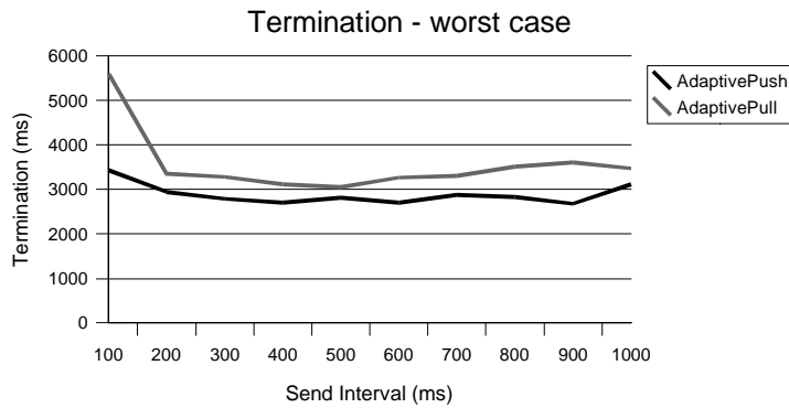
Figure 10 - Adaptive detectors: worst case comparison
