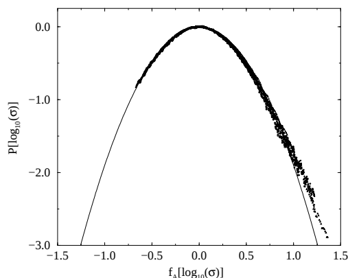
FIG. 10: Same distributions as in the previous figure in the reduced variable f_A(g) = (\sqrt{1 + 2Kg} - 1) / KA where g = \log_{10}(\sigma) and K = 0.25 . The data collapse onto a simple parabola, which shows the Gaussian character of the distribution of f_A(g)
