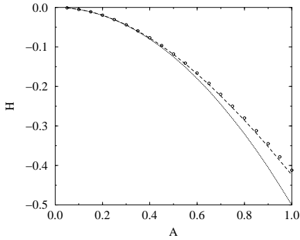
FIG. 11: Offset H of the equivalent boundary from the geometrical average of a sine profile of variable amplitude A and fixed wavelength \lambda = 2\pi . The dotted line is the result of the perturbation analysis, Eq.(43) and the symbols are the results obtained from a conformal mapping. The dashed curve is the proposed fit Eq.(46).
