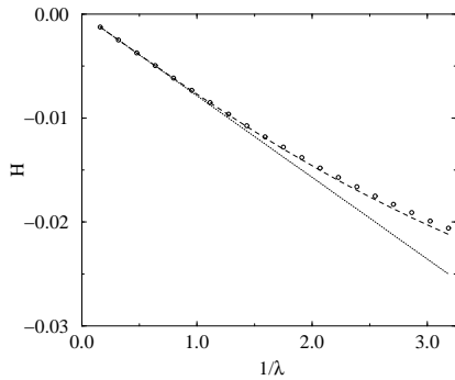
FIG. 12: Offset H of the equivalent boundary from the geometrical average of a sine profile of amplitude A = 0.05 and variable wavelength \lambda . The dotted line is the result of the perturbation analysis, Eq.(43) and the symbols are the results obtained from a conformal mapping. The dashed curve is the proposed fit Eq.(46).
