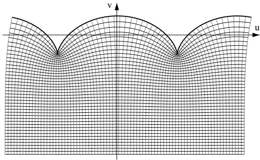
FIG. 2: Image of a regular square grid of the semi-plane \mathcal{D} using the transformation (7). The parameter \omega has been set to its maximum value of 1. Cusp appears on the boundary.
