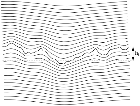
FIG. 10: Schematic illustration of the finite “electrical” thickness of a rough equipotential. The rough equipotential C (shown as a bold curve) is placed in between two remote planar electrodes. The presence of the rough equipotential reduces the resistance of the medium in a similar way as an planar equipotential with a finite thickness. Extrapolating the far electrical field from the remote electrodes gives “equivalent” smooth boundaries shown as dotted lines. Their relative distance defines the “electrical” thickness h_t .
