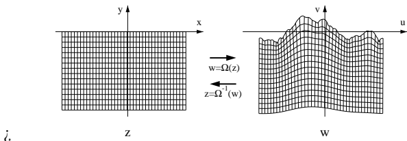
FIG. 1: Illustration de la transformation conforme \Omega introduite dans cette section. A schematic illustration of the mapping \Omega which maps the semi-infinite plane \mathcal{D} onto the domain limited by a rough interface \mathcal{E} .
