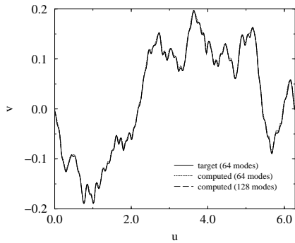
FIG. 7: An example of the obtained profile \partial\mathcal{E} from the conformal map, compared to the objective one, chosen to be a self-affine function with a roughness exponent \zeta = 0.8 . The amplitude of the profile is 95% of the maximum amplitude which preserves the convergence of the algorithm.
