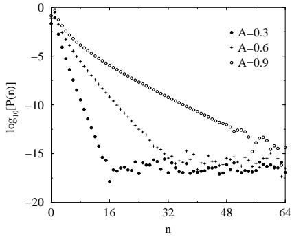
FIG. 3: Power spectrum of the function \omega computed for a sine profile. The three curves corresponds to three amplitudes, A = 0.3 ( \bullet ), 0.6 ( + ) and 0.9 ( \circ ).
