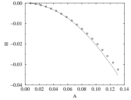
FIG. 13: Offset H of the equivalent boundary from the geometrical average of a self-affine profile of variable amplitude A , a roughness exponent \zeta = 0.8 and 16 modes. The dotted line is the result of the perturbation analysis, Eq.(49) and the symbols are the results obtained from a conformal mapping.
