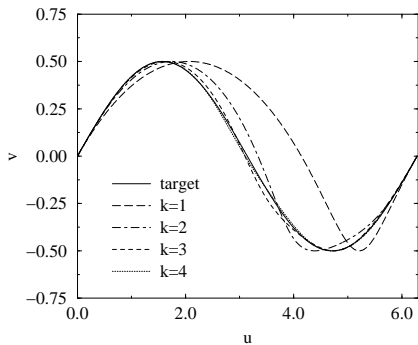
FIG. 4: Images of the real axis obtained after the first k iterates of the algorithm with the objective profile ( h(u) = A \sin(u) ) shown as a bold line. In this particular example A = 0.5 and the number of modes is 32.
