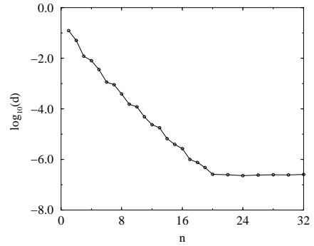
FIG. 5: Minimum error obtained using the algorithm described in the text for computing the conformal map on a sine profile with amplitude A = 0.5 , as a function of the number n of modes used in \omega .
