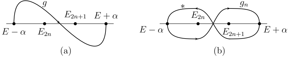
Figure 12: The curves g and \tilde{g}_n
