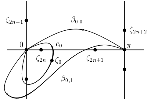
Figure 11: The curve c_0
