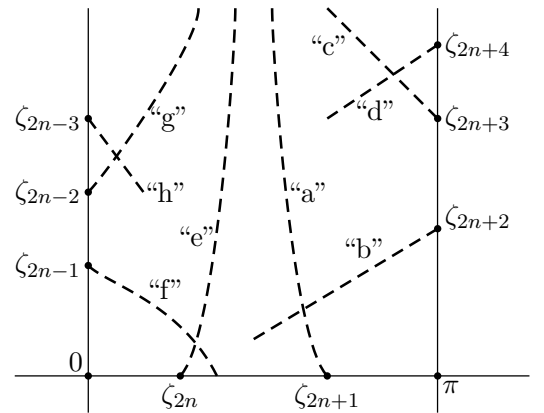
Figure 8: The Stokes lines
