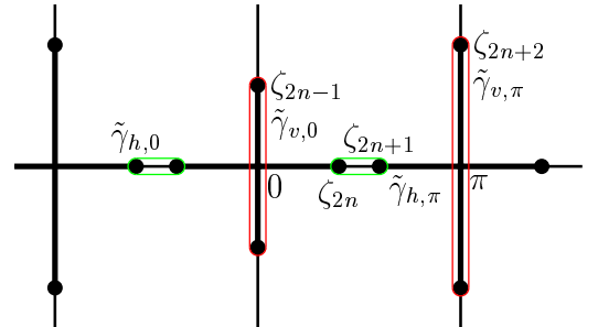
Figure 4: The loops for the phases
