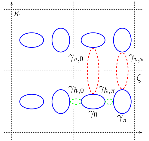
Figure 2: The adiabatic phase space
