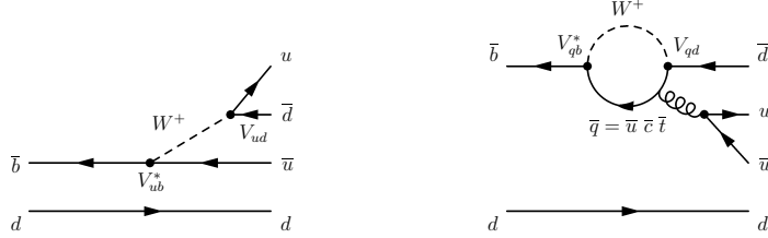
Figure 1: Tree (left) and penguin (right) diagrams for the decays B^0 \rightarrow \pi^{\pm}\pi^{\mp} , B^0 \rightarrow \rho^{\pm}\pi^{\mp} and B^0 \rightarrow \rho^{\pm}\rho^{\mp} .
