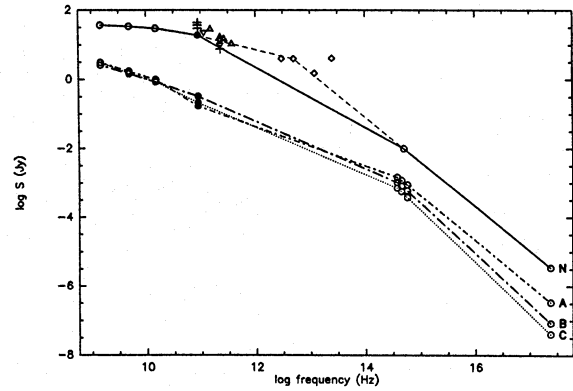
Fig. 4. Spectra of the nucleus and knots of the jet. All values for the nucleus have been multiplied by 10 for clarity of the plot. Straight lines connect individual data points for a given feature. Knot A: dash-dot line; knot B: long dash-dot line; knot C: dotted line. For the nucleus, the solid line connects high resolution measurements while the dashed line includes the 5000 GHz ( 60 \mu\text{m} ) IRAS point as well. The black dots ( \bullet ) are from the present work and open circles ( \circ ) are values taken from Biretta et al. (1991). Low resolution values are from + : Steppe et al. (1988); \nabla : Braine & Wiklind (1993); \triangle : Knapp & Patten (1991); \square : Salter et al. (1989); \diamond : Young et al. (1989).
