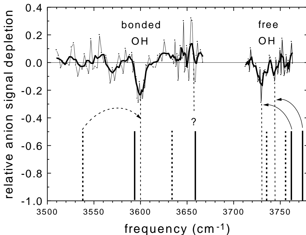
Figure 1: IR spectrum of the mass-selected neutral water dimer obtained from DBA signal depletion. Small squares correspond to relative depletion values averaged over three independent measurements while full thick lines correspond to a smooth over three adjacent points. Experimental line positions are indicated by thin dash lines and theoretical frequencies are located by full (anharmonic) or dash (scaled harmonic) bars. The question mark corresponds to the position of the fourth line, expected from matrix data. See text for discussion.
