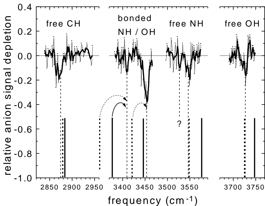
Figure 2: As in Fig. 1 for mass-selected neutral formamide-water complex. The question mark corresponds to a line which is not assigned. See text for discussion.
