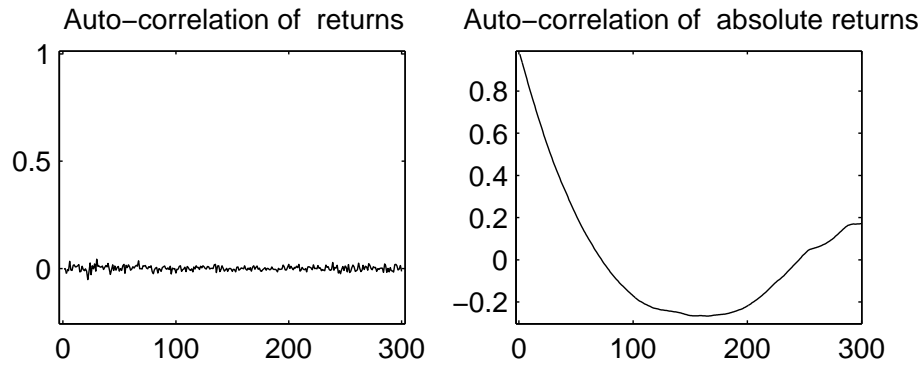
Figure 7: Numerical simulation of the model with s = 0.015 N = 1500 \lambda = 0.1 D = 10^{-5}
