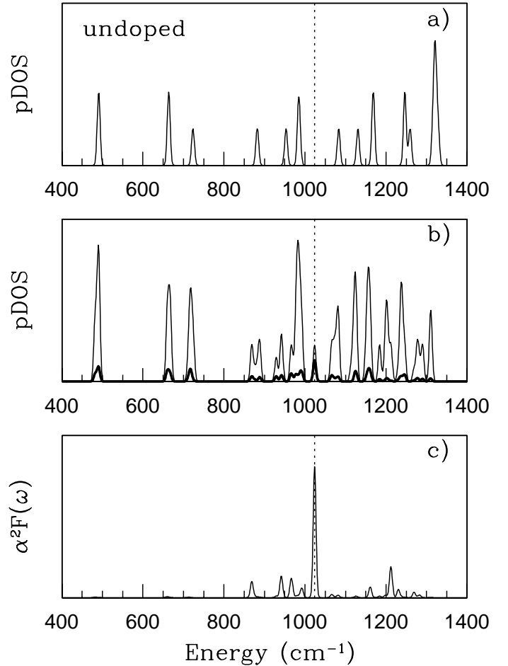
FIG. 2. Phonon density of states p\text{DOS} for (a) bare diamond with modes on an unshifted (3\times 3\times 3) grid (b) the boron doped \text{BC}_{53} cell with modes at \Gamma . In (c) the spectral function \alpha^2F(\omega) is represented for modes at \Gamma . Energies are in \text{cm}^{-1} and the y-axis magnitude is arbitrary. A 5\text{ cm}^{-1} broadening has been used. The vertical dotted lines indicate the energy position of the 3-fold B-related vibrational modes.
