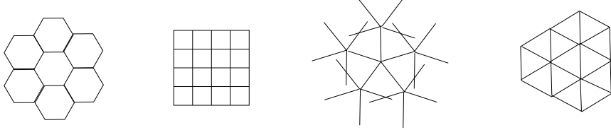
Figure 5 : N -holomorphic functions
