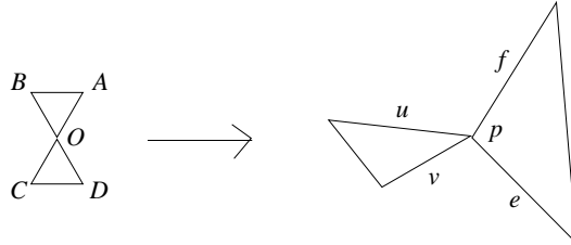
Figure 6 : Two triangles
