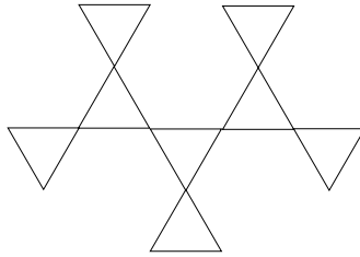
Figure 1 : The graph Tr_3
