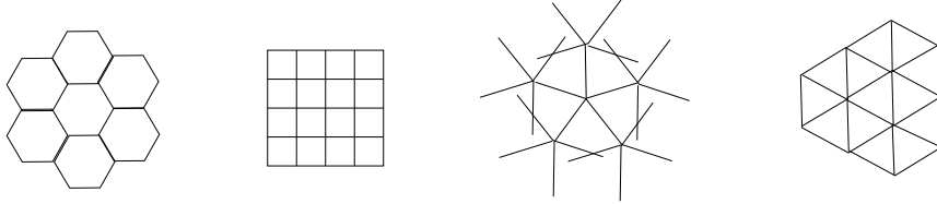
Figure 5 : N -holomorphic functions
