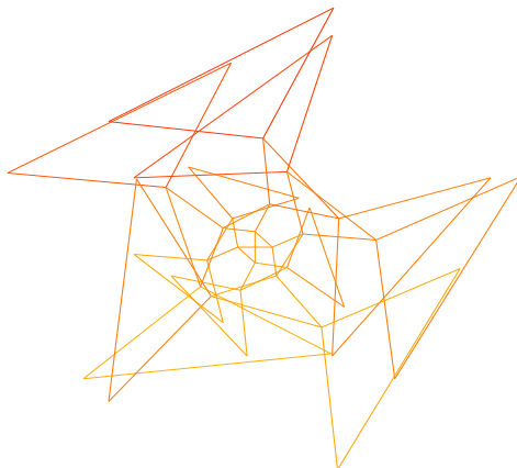
Figure 8 : Images of balls in Tr_3 of radius 3 and 5 by holomorphic functions
