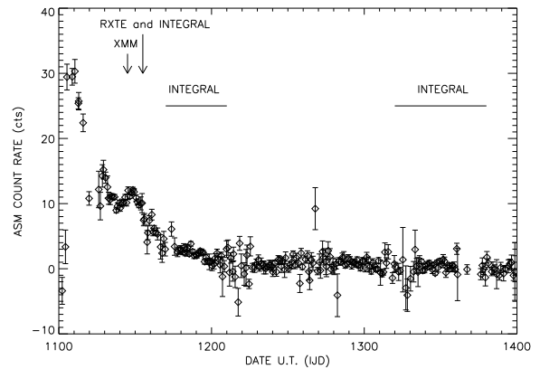
Figure 1. RXTE/ASM light curve (2-12 keV) of the outburst of XTE J1720-318. The arrows show the dates of the XMM-Newton, RXTE and INTEGRAL simultaneous observations. The approximate periods of later INTEGRAL observations are indicated by horizontal lines. The universal time is in units of INTEGRAL Julian Days (IJD) where IJD = MJD - 51544 days.
