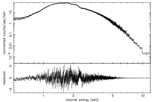
Figure 6. XMM-Newton/EPIC-PN spectrum of XTE J1720-318. The best-fit model, an absorbed MCD plus a power law, is over plotted as a solid line. Residuals (in counts s -1 keV -1 ) are also shown.
