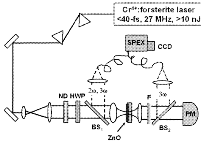
Figure 2. Experimental set-up for the third-harmonic generation. BS 1,2 - are dichroic beamsplitters, ND - neutral density filter wheel, F - blue transmitting, near-IR absorbing filter, PM - power meter, HWP - half-wave plate.
