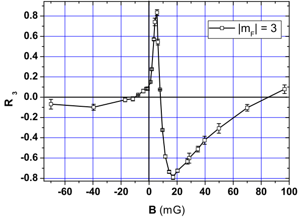
FIG. 7: Ratio R_{03} as a function of the magnetic field. It represents a Feshbach resonance for |m_F| = 3 . This resonance has a more simple shape. Assuming that it is a simple resonance we go to simulate the scattering process.
