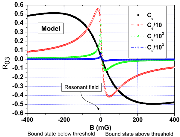
FIG. 8: For \Gamma_i = 0 . For large values of C_e , the shape and the (“natural”) width of the resonance is determined by C_e . The resonance has a symmetrical dispersive shape. For small values of C_e , the shape and the width of the resonance is determined by the collision energy distribution. The line shape shows a strong asymmetry. The calculation clearly indicates that the top of the sharp feature corresponds to the magnetic field that meets the resonant condition.
