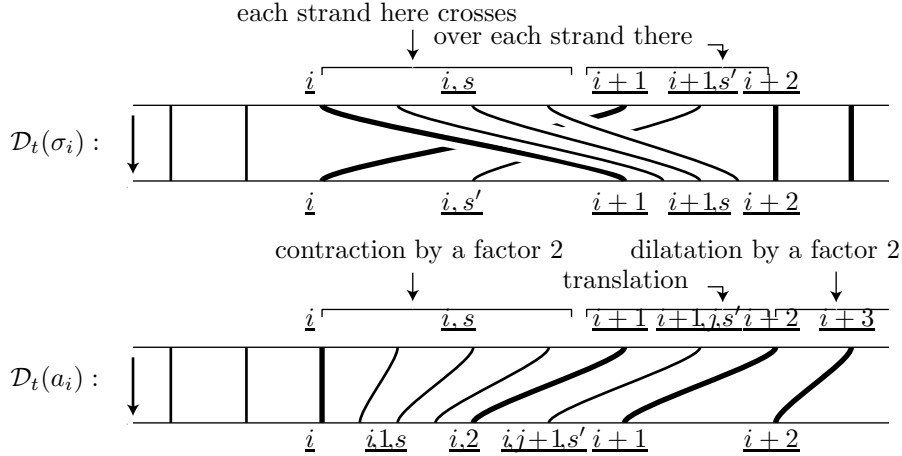
FIGURE 4. The diagrams \mathcal{D}_t(\sigma_i) and \mathcal{D}_t(a_i) : in \mathcal{D}_t(\sigma_i) , the positions in [\underline{i}, \underline{i + 1}) and in [\underline{i + 1}, \underline{i + 2}) are exchanged (with a contraction/dilatation factor 2 due to the dyadic realization); in \mathcal{D}_t(a_i) , the positions in [\underline{i}, \underline{i + 1}) are contracted by 2, those in [\underline{i + 1}, \underline{i + 2}) are translated to the left, and those in [\underline{k}, \underline{k + 1}) are translated to the left and dilated by 2. In terms of positions viewed as sequences of integers, \mathcal{D}_t(\sigma_i) exchanges (i, s) and (i + 1, s) for every sequence s , while \mathcal{D}_t(a_i) connects (i, s) to (i, 1, s) , then (i + 1, j, s) to (i, j + 1, s) , and (k, s) to (k - 1, s) for k > i + 1 .
