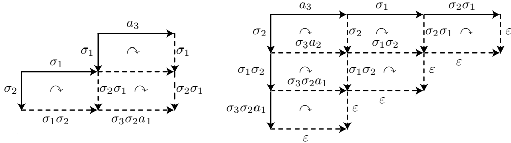
FIGURE 19. Right cube condition for the triple (\sigma_2, \sigma_1, a_3) : one first reverses \sigma_2^{-1} \sigma_1 \sigma_1^{-1} a_3 to a positive-negative word, here \sigma_1 \sigma_2 \sigma_3 \sigma_2 a_1 \sigma_1^{-1} \sigma_2^{-1} \sigma_1^{-1} , and, then, one checks that a_1^{-1} \sigma_2^{-1} \sigma_3^{-1} \sigma_2^{-1} \sigma_1^{-1} \sigma_2^{-1} a_3 \sigma_1 \sigma_2 \sigma_1 is right reversible to \varepsilon .
