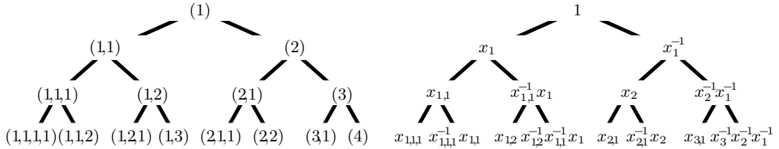
FIGURE 16. Addresses for the nodes in trees, and the associated natural F_{\bullet} -colours; for each s , the variable x_s is the natural colour of the node with address (s, 1)
