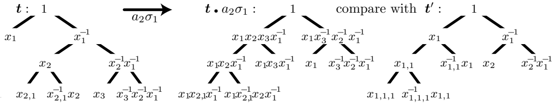
FIGURE 17. Computing the automorphism of F_\bullet associated with a_2 \sigma_1 : we let a_2 \sigma_1 act on a tree \mathbf{t} with natural F_\bullet -colours, and compare the colours in \mathbf{t} \cdot a_2 \sigma_1 with the natural ones: the node with natural colour x has colour \psi(a_2 \sigma_1)(x) in \mathbf{t} \cdot a_2 \sigma_1 . For instance, x_1 is mapped to x_1 x_2 x_3 x_1^{-1} and that x_{1,1}^{-1} x_1 is mapped to x_1 x_3 x_1^{-1} .
