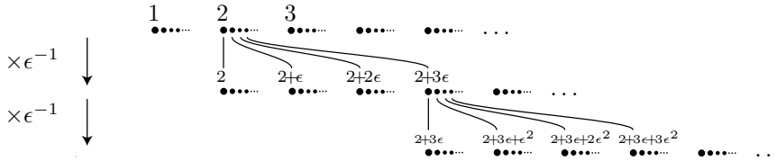
FIGURE 1. The set of all positions realized using infinitesimal distances
