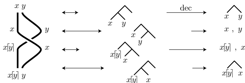
FIGURE 11. Correspondence between sets of S -coloured positions and S -coloured trees: here we start from \underline{1} and \underline{1,2} coloured x and y , i.e. , from the coloured tree (\bullet_x \bullet_y) \bullet ; then we go to \underline{1} and \underline{2} coloured x and y , i.e. , to \bullet_x (\bullet_y \bullet) , etc. ; on the right, we show the right decomposition of the trees, i.e. , the subtrees under the right branch, the last leaf excepted
