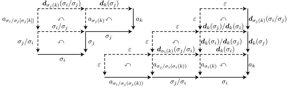
FIGURE 18. Left cube condition for the triples (\sigma, \sigma, a) : one first reverses \sigma_i \sigma_j^{-1} \sigma_j a_k^{-1} to (\sigma_j / \sigma_i)^{-1} (a_{\sigma_i / \sigma_j [\sigma_j [k]])^{-1} (d_{\sigma_j [k]}(\sigma_i / \sigma_j)) (d_k(\sigma_j)) , then restart from (a_{\sigma_i / \sigma_j [\sigma_j [k]]) (\sigma_j / \sigma_i) (\sigma_i) (\sigma_k)^{-1} (d_k(\sigma_j))^{-1} (d_{\sigma_j [k]}(\sigma_i / \sigma_j))^{-1} and check that the latter is left reversible to \varepsilon ; the values follow from (7.2) and the fact that the permutations associated with (\sigma_i / \sigma_j) \sigma_j and (\sigma_j / \sigma_i) \sigma_i coincide, as both come from the left lcm of the involved braid.
