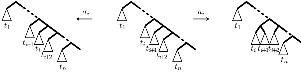
FIGURE 5. Action of \sigma_i and a_i on a tree: \sigma_i switches the i th and the (i+1) st factors in the right decomposition, while a_i glues them.
