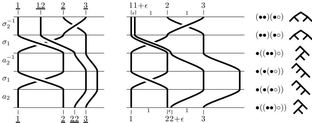
FIGURE 6. The dyadic realization of the diagram \mathcal{D}_{(\bullet\bullet)(\bullet\bullet)}(\sigma_2^{-1}\sigma_1 a_2^{-1}\sigma_1 a_2) and its infinitesimal version, which is of course topologically equivalent; at each step, the corresponding set of positions is displayed, both as a parenthesized expression (the last node is marked \circ because it contributes no position) and as a binary tree.
