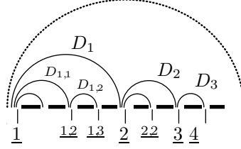
FIGURE 13. The disks D_s : essentially, D_s is the disk based on s and its immediate successor in the lexicographical ordering: for instance, D_1 is the disk with diameter [1, 2] , D_{1,1} is the disk with diameter [1, 1.2] (which is [1.1, 1.2] ); the adjustment guarantees that the disks D_{s,i} are disjoint and nested in D_s
