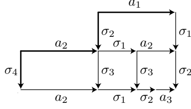
FIGURE 10. Right reversing diagram for \sigma_4^{-1}a_2\sigma_2^{-1}a_1 : one starts with a staircase labelled \sigma_4^{-1}a_2\sigma_2^{-1}a_1 by drawing a vertical x -labelled arrow for each letter x^{-1} , and an horizontal y -labelled arrow for each positive letter y . Then, when x^{-1}y is replaced with vu^{-1} , we complete the open pattern corresponding to x^{-1}y into a square by adding horizontal v -labelled arrows and vertical u -labelled arrows.
