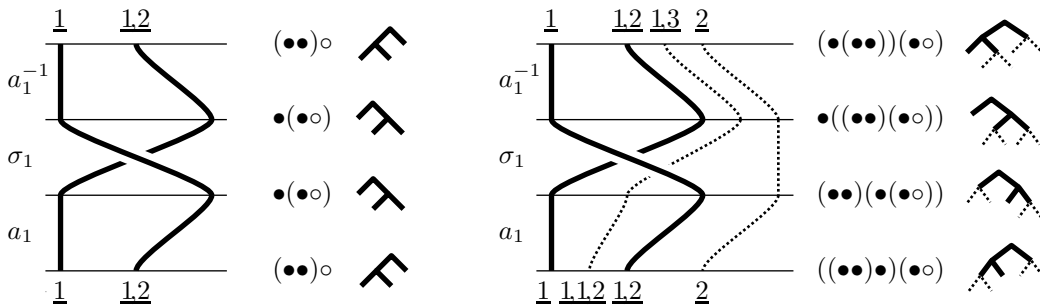
FIGURE 8. Completion of \mathcal{D}_{(\bullet\bullet)\bullet}(a_1^{-1}\sigma_1 a_1) into \mathcal{D}_{(\bullet(\bullet\bullet))(\bullet\bullet)}(a_1^{-1}\sigma_1 a_1) : two more leaves in the tree, two more strands in the braid
