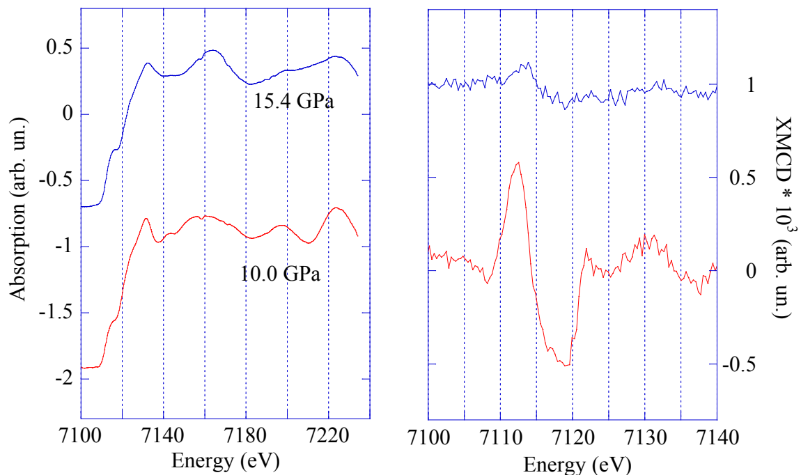
Figure3: Fe-K edge XAS (left panel) and XMCD (right panel) signals of pure Fe foil recorded at 10 and 15.4 GPa. The small
