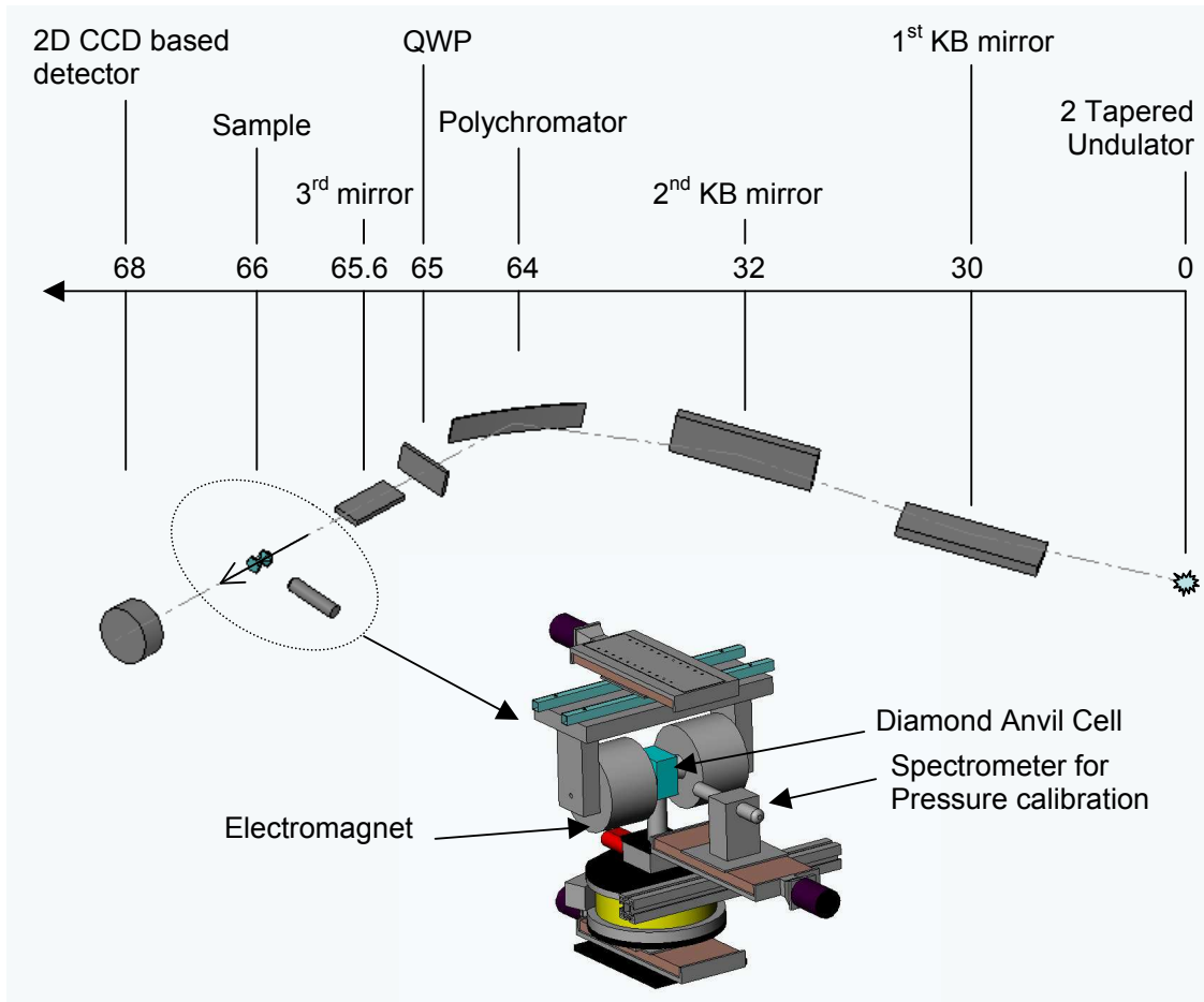
Figure 1 : ID24 optical scheme and sample environment for XMCD at high pressure (not scaled).
