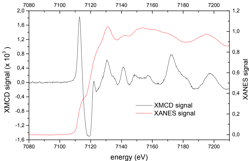
Figure 2 : XAS and XMCD signal recorded on ID24 at the K edge of a pure Fe foil out of the pressure cell.
