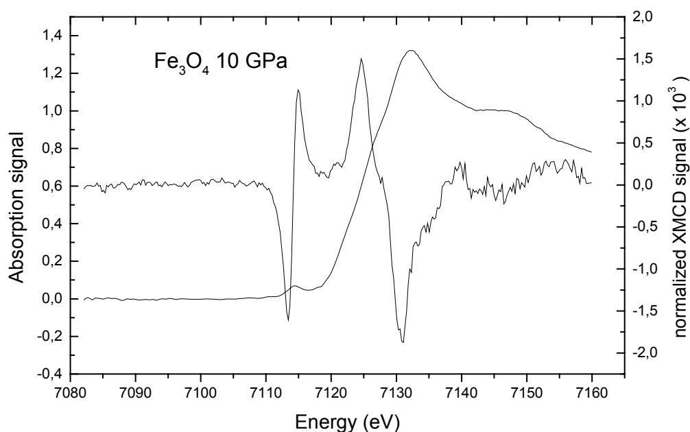
Figure 5 : Fe K edge XMCD and XANES signals measured at 10 GPa on \text{Fe}_3\text{O}_4 .
