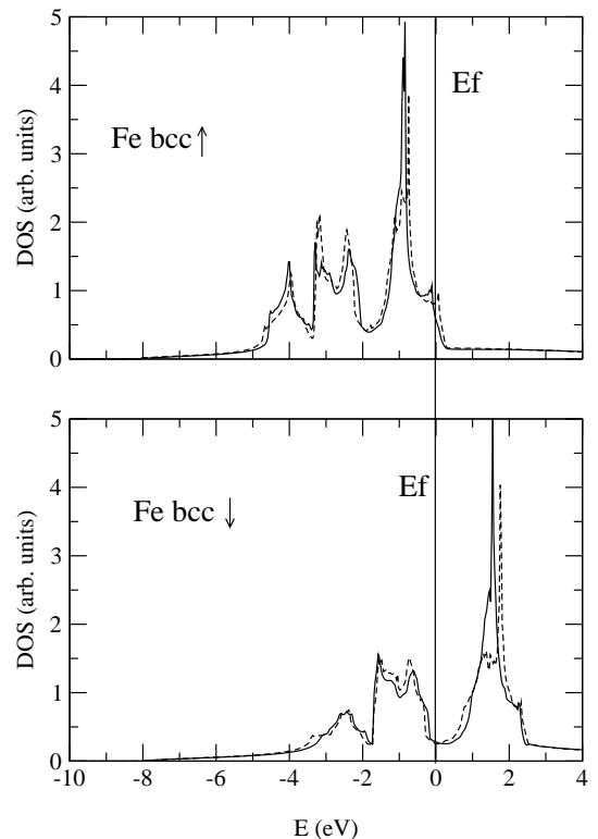
FIG. 8: Density of states as obtained for bcc Fe in the tight-binding Hartree-Fock model (solid lines, V_0 = 0.5 eV), and in the band structure calculation using the FLAPW method of Ref. 24 (dashed lines) for \uparrow -spin electrons (top), and \downarrow -spin electrons (bottom) in the FM ground state.
