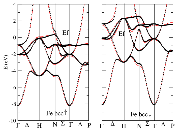
FIG. 9: Electronic structure as obtained for bcc Fe in the tight-binding Hartree-Fock model ( V_0 = 0.5eV , black triangles), and in the band structure calculation using the FLAPW method of Ref. 24 (solid lines) for \uparrow -spin electrons (left), and \downarrow -spin electrons (right) in the FM ground state.
