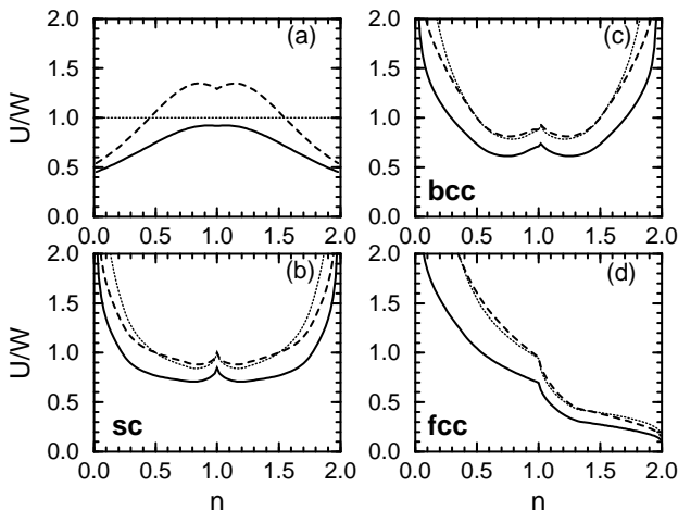
FIG. 2: Critical value of U/W ( W : unrenormalized band width) above which the SF phase becomes stable as a function of the band filling n and for: (a) constant density of states, (b) sc lattice, (c) bcc lattice, and (d) fcc lattice. The meaning of different lines and the parameters are the same as in Fig. 1.
