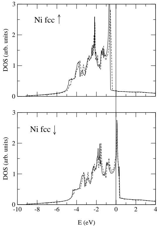
FIG. 12: Same caption as in Fig. 8, but for fcc Ni.
