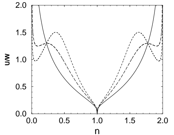
FIG. 5: Critical value of U/W ( W : unrenormalized band width) for the onset of the Stoner instability in a bcc lattice with an s band as a function of the band filling n for increasing values of V/U (0: full line, 0.35: dashed line, 0.55: dotted line) and J = J' = 0 .
