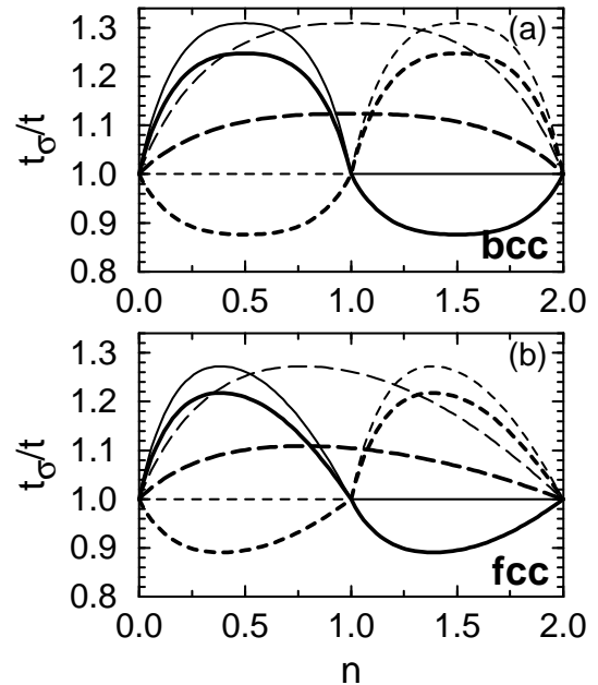
FIG. 3: Effective hopping integrals t_\sigma (in units of t ) as a function of the band filling n of an s band for: (a) bcc and (b) fcc lattices. Different lines refer to: PM phase (long dashed lines), t_1/t (full lines) and t_1'/t (dashed lines) in the SF phase (stable at sufficiently large U , see Fig. 2). The parameters are: V = 0.15W ( W = 16t ), J' = J , and: J = 0 (thin lines), J = 0.03W (heavy lines).
