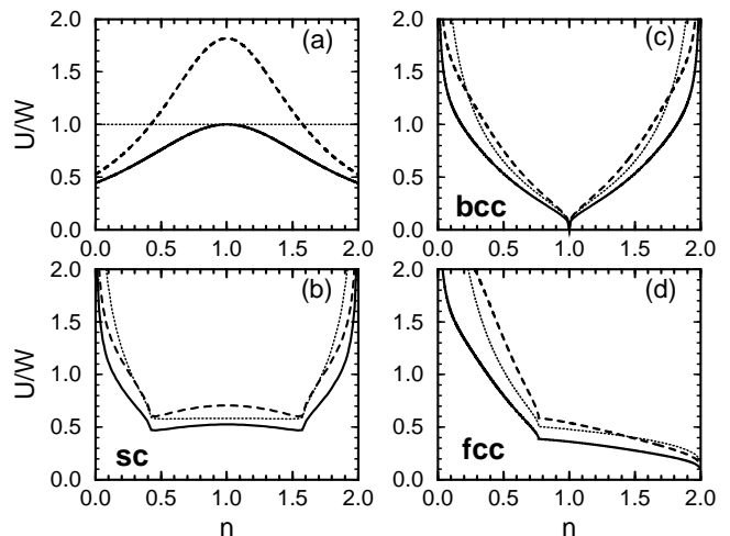
FIG. 1: Critical value of U/W ( W : unrenormalized band width) for the onset of the Stoner instability as a function of the band filling n for an s band and: (a) constant density of states, (b) sc lattice, (c) bcc lattice, and (d) fcc lattice. Different lines correspond to: V = J = 0 (dotted lines); V = 0.15U , J = 0 (dashed lines); V = 0.15U , J = 0.03U ( J' = J ) (solid lines).
