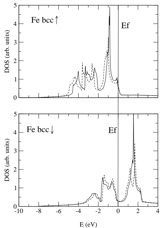
FIG. 6: Density of states as obtained for bcc Fe in the tight-binding Hartree-Fock model with (solid lines, V_0 = 0.5eV ) and without (dashed lines) Coulomb inter-site interaction, for \uparrow -spin electrons (top), and \downarrow -spin electrons (bottom) in the FM ground state.
