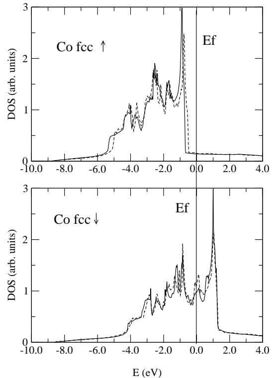
FIG. 11: Same caption as in Fig. 8, but for fcc Co.
