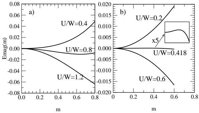
FIG. 4: Magnetic energy E_{mag} (in units of the unrenormalized band width W ) as a function of the magnetic moment m for a fcc lattice with an s band for two band fillings (a) n = 0.9 (b) n = 1.4 and increasing values of U/W . The other parameters are V = 0.15U , J = J' = 0 . The inset shows the case n = 1.4 , U/W = 0.418 with an enlarged energy scale, proving that the PM state is metastable.
