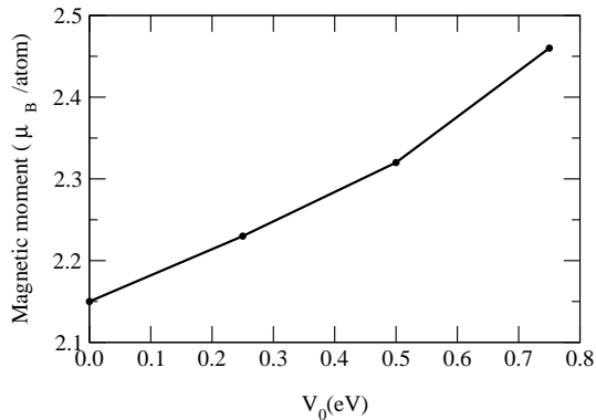
FIG. 7: Variation of the magnetic moment of bcc Fe as a function of the Coulomb inter-site interaction V_0 .
