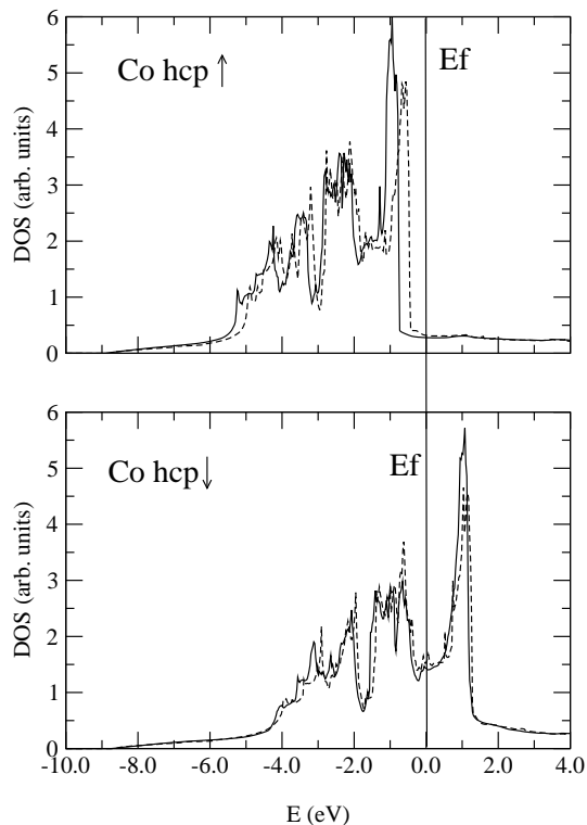
FIG. 10: Same caption as in Fig. 8 but for hcp Co.
