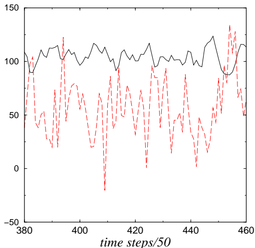
Figure 4: Time evolution of K (continuous line) and K' (dotted line, shifted by -100), with an enlarged time scale. Same conditions as for Fig.3
