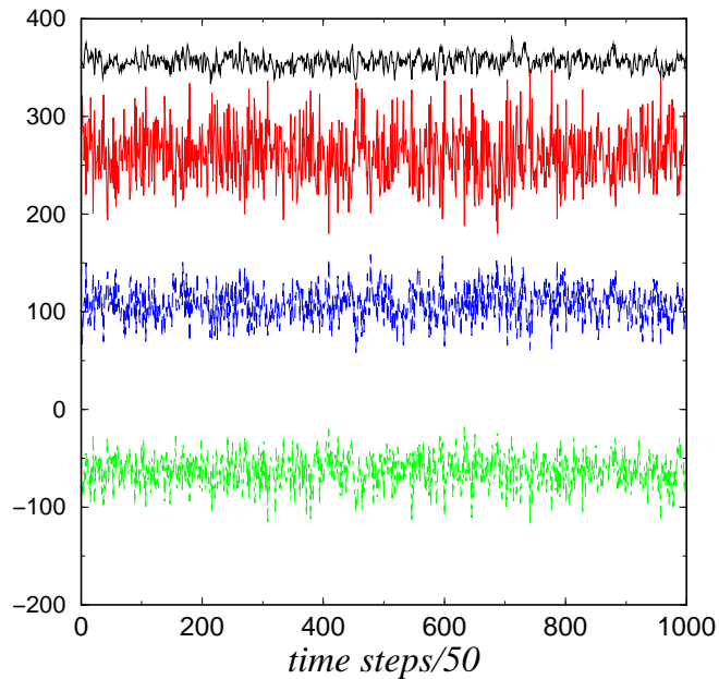
Figure 3: Time evolution of various quantities at a density of \rho = 0.35 and excitation energy per particle of E^*/N = 4.0 . From top to bottom: K (shifted by 250 units), K' (shifted by 100 units), \sum_i(V_i - B_i) and \sum_{i<j} V_{i,j} .
