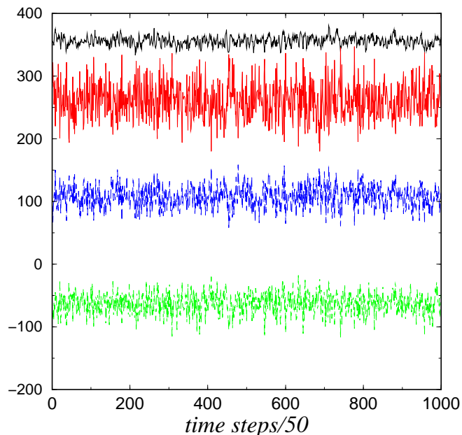
Figure 3: Time evolution of various quantities at a density of \rho = 0.35 and total energy per particle of E/N = 4.0 . From top to bottom: K (shifted by 250 units), K' (shifted by 200 units), \sum_i(V_i - B_i) and \sum_{i<j} V_{i,j} .
