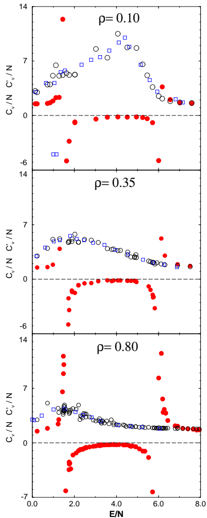
Figure 2: The heat capacity c_v/N (open circles and open squares, see text) and the quantity c'_v/N (filled circles), as a function of the total energy (in units \epsilon of the Lennard-Jones potential) for isochore paths at \rho = 0.10, 0.35 and 0.80 .
