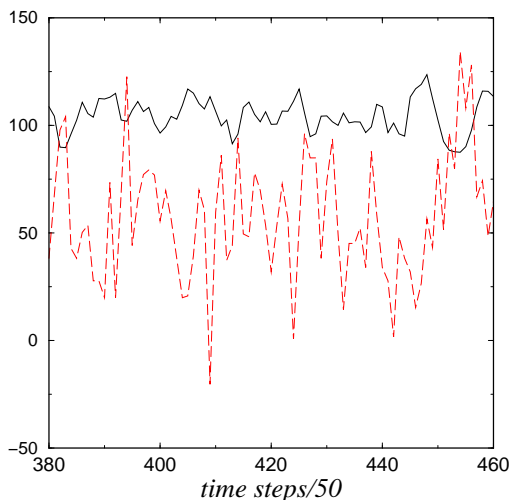
Figure 4: Time evolution of K (continuous line) and K' (dotted line), with an enlarged time scale. Same conditions as for Fig.3
