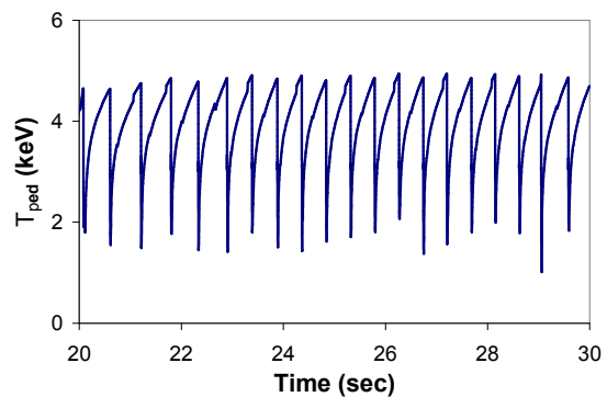
Figure 2: Ion temperature at the top of the pedestal is plotted as a function of time. A decrease in pedestal temperature indicates an ELM crash.
