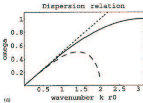
FIG. 5: The LDLW dispersion relation: frequency \omega_L vs. wavenumber k (solid curve). We have also depicted: the continuous approximation (dashed curve) and the acoustic (tangent) curve at the origin.
