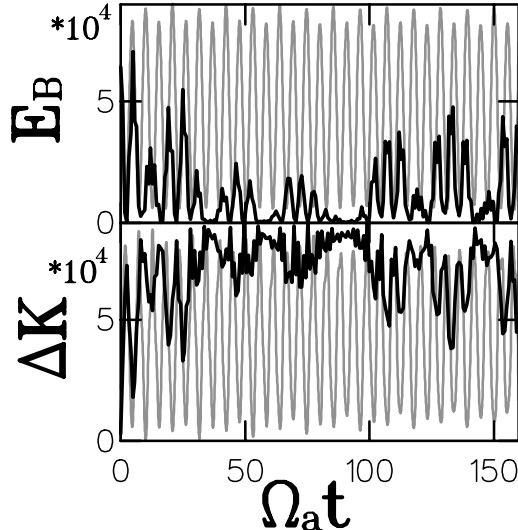
Figure 3: Time variations of total magnetic-field energies and ion kinetic energies. The thin and thick lines represent single- and four-ion-species plasmas, respectively.
