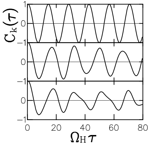
Figure 2: Autocorrelation functions of the fluctuations with k\rho_H = 0.1 in the same plasmas as shown in Fig. 1
