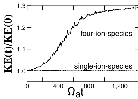
Figure 5: Long time variations of ion kinetic energies in the single- and four-ion-species plasmas.
