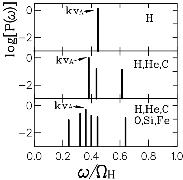
Figure 1: Power spectra of magnetic field fluctuations with k\rho_H = 0.1 in three different plasmas.
