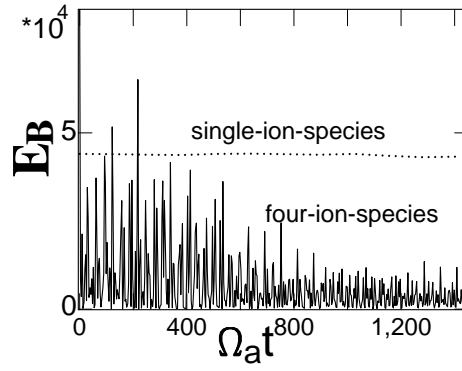
Figure 4: Long time variations of total magnetic-field energies. The solid line and dashed lines represent the energies in the four- and single-ion-species plasmas, respectively. For the single-ion-species plasma, the values averaged over the time period t = 2\pi/k_0v_A are plotted.
