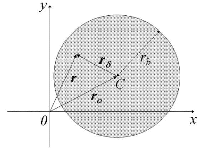
FIG. 1: Schematic of the beam distribution of Eq. (12) and corresponding vectors. C corresponds to the centroid position.
