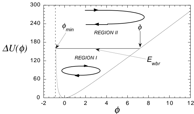
FIG. 1: Oscillating ( I ) and wave breaking ( II ) regions for the electric potential at \psi = 0 . \Delta U is defined in the text.
