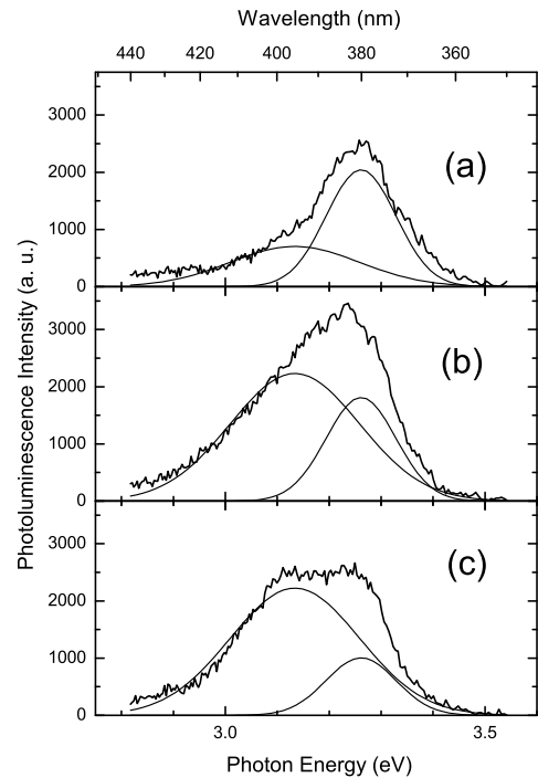
FIG. 4: Evolution of the PL spectra of gas-suspended ZnO nanoclusters. The oxygen pressure was 8 mbar. (a) 1st pass (0 minutes); (b) 2nd pass (delay 3 min); (c) 3rd pass (delay 6 min). The fluence of ArF laser was \sim 30 \text{ mJ/cm}^2 . Thin lines show the results of fitting by two Gaussians.
