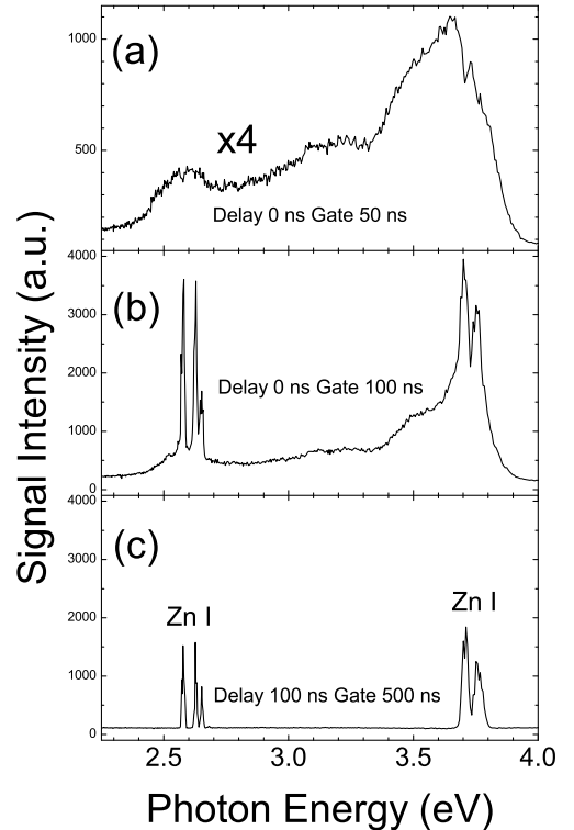
FIG. 2: Fragmentation of gas-suspended ZnO nanoclusters excited by ArF laser (fluence \sim 200 \text{ mJ/cm}^2 ): (a) Boxcar delay 0 ns, gate 50 ns; (b) delay 0 ns, gate 100 ns; (c) delay 100 ns, gate 500 ns. The oxygen pressure was 4 mbar. The atomic lines of Zn are indicated in the figure. The observation point was at a distance of \sim 5 \text{ cm} from the target.
