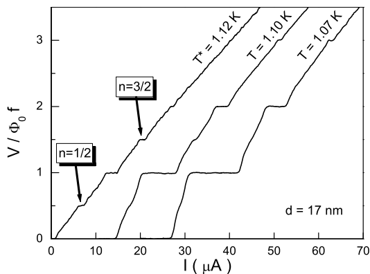
FIG. 4: Shapiro steps in the voltage-current curve of a 17 nm thick junction with an excitation at 800 kHz (amplitude about 18 \mu\text{A} ). Half-integer steps ( n=1/2 and n=3/2 ) appear at the 0-\pi crossover temperature T^* . Curves at 1.10 and 1.07 K are shifted by 10 and 20 \mu\text{A} for clarity.
