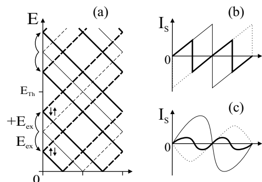
FIG. 1: (a) Energy of Andreev levels versus phase difference in a one-dimensional ballistic junction ( E_{Th} = \hbar v_F/d \ll \Delta ) [4]. Each state of the normal case (thin lines) is split by the exchange energy E_{ex} of the ferromagnet (thick lines). The states in solid (dashed) lines carry positive (negative) currents. (b) Current-phase relation for this model at zero temperature in the normal case (thin line), in \pi junctions (dotted line) and at the crossover (thick line). (c) Current-phase relation in diffusive regime for the same situations.
