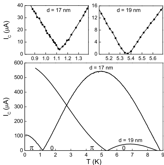
FIG. 2: Temperature dependence of the critical current for two Nb/Cu 52 Ni 48 /Nb junctions. Upper graphs are expanded views near the crossovers between 0 and \pi states: the critical current has a non-zero (zero) minimum for the 17 nm (19 nm) thick junction.
