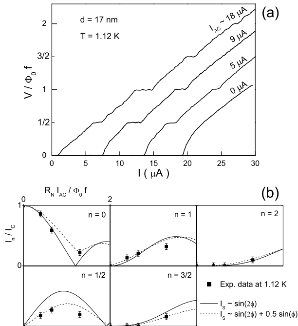
FIG. 5: (a) Shapiro steps in the voltage-current curves of the 17 nm thick junction at 1.12 K with an excitation at 800 kHz. Excitation amplitudes are about 18, 9, 5 and 0 \mu\text{A} . The respective curves are shifted by 0, 5, 10 and 15 \mu\text{A} for clarity. (b) Width of the integer and half-integer steps versus normalized amplitude of the alternative current. Experimental values (symbols) are compared with numerical simulations for two current-phase relations containing a dominant \sin(2\phi) component (lines). All graphs have same axis and scales.
