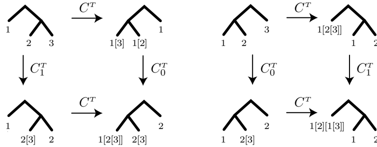
FIGURE 18. The twisted C -geometric relations
