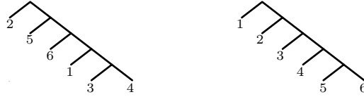
FIGURE 10. The coloured right vines \langle \{2, 5, 6\}, \{1, 3, 4\} \rangle and \langle \{2, 5, 6, 1, 3, 4\} \rangle ; the latter is also \langle \{1, 2, 3, 4, 5, 6\} \rangle
