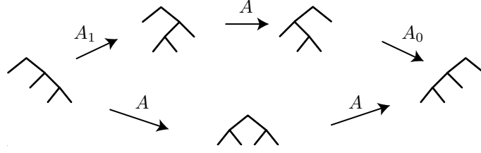
FIGURE 5. The pentagon relation
