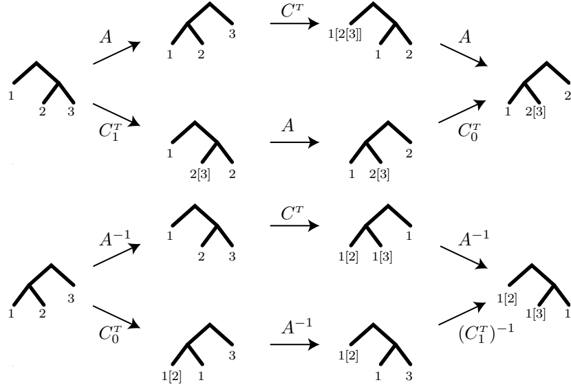
FIGURE 17. The twisted hexagon relations
