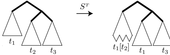
FIGURE 13. The twisted semi-commutation operator S^T
