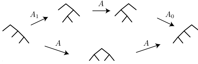
FIGURE 5. The pentagon relation
