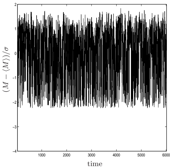
FIG. 13: Metropolis evolution of m at T_c(L) .
