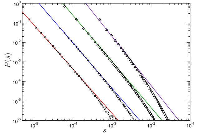
FIG. 10: Clusters size distribution at T^*(L) for L = 64(\Delta) , 128(\diamond) , 256(+) and 512(\times) . The solid lines are the best power laws obtained.
