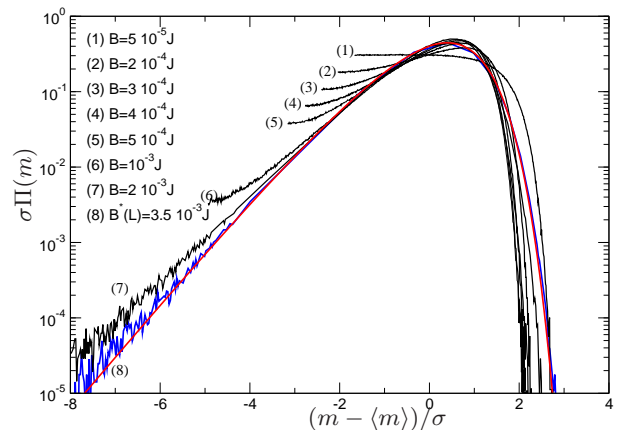
FIG. 3: PDF for a subsystem L = 32 , in system of size L_0 = 128 , for various values of the magnetic field B at T_c(L = 128) . The plain curve is the PDF for the 2D-XY model.
