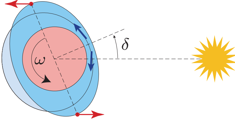
Figure 5. Atmospheric tides
