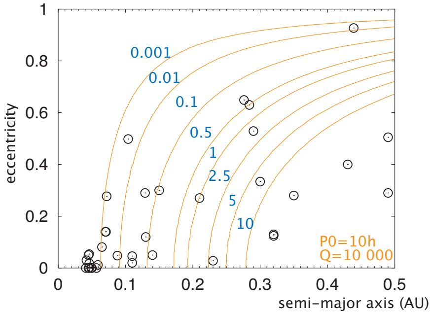
Figure 4. Tidally evolved planets with Q = 10^4 and initial period P_0 = 10 \text{ h} .
