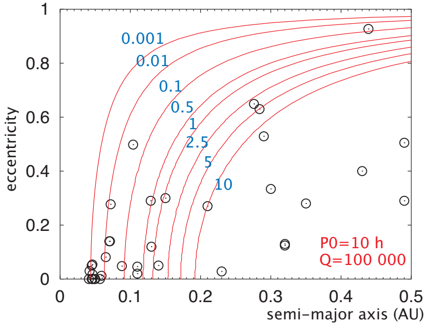
Figure 3. Tidally evolved planets with Q = 10^5 and initial period P_0 = 10 \text{ h} . The labelled curves denotes (in Gyr) the time needed to reach the equilibrium.
