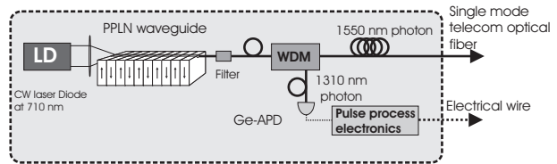
Fig. 1. Schematic of our Heralded Single Photon Source. It has an electrical output which allows heralding the arrival of a single photon at the single mode optical fiber output.
