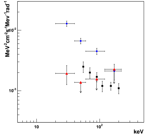
Figure 6. Residual Galactic flux. The blue circles give the total source spectrum, the red triangles the remaining emission possibly of diffuse origin and the black squares give the estimated interstellar emission taking into account SIGMA sources (Purcell et al. 1996; Kinzer et al. 1999). The diffuse spectrum is consistent with the one obtained by SPI with the same source list (Strong et al. 2004)
