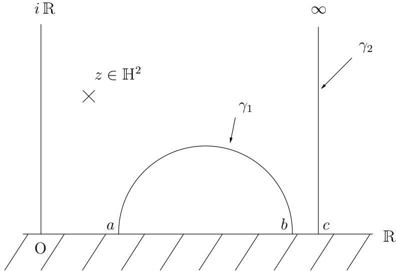
Figure 1: \mathbb{H}^2 and its geodesics
