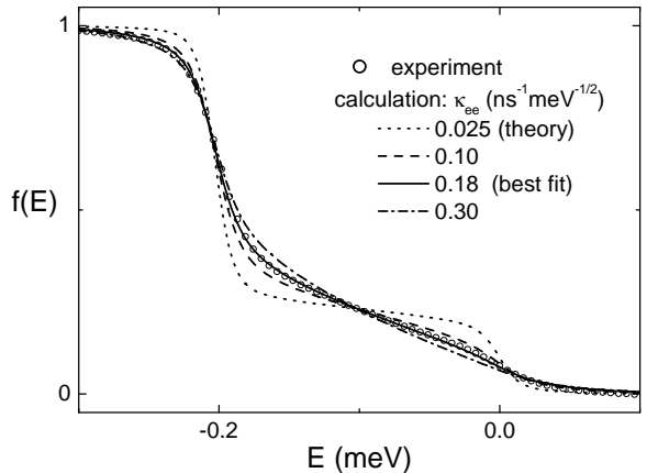
Fig. 7. Measured (o) distribution function f_{1/4}(E) in the “conventional” Relax experiment using sample AgXII40 with the switch of FIG. 6 in position 1, and for U = 0.2 mV. The solid line is a numerical solution to the Boltzmann equation using the prefactor \kappa_{ee} = 0.18 \text{ ns}^{-1} \text{ meV}^{-1/2} for the Coulomb interaction between electrons. As shown by the three dot-dashed lines, other values of \kappa_{ee} produce markedly worse fits to the data. In particular, the theoretical value \kappa_{ee} = 0.025 \text{ ns}^{-1} \text{ meV}^{-1/2} does not come close to reproducing the experimental results.
