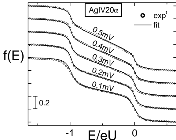
Fig. 3. Measurements ( \circ ) and fits (solid curves) of the quasiparticle energy distribution function f_{\frac{1}{2}}(E) for five different values of the applied voltage U across the wire AgIV20 \alpha . The data have been shifted vertically for clarity.
