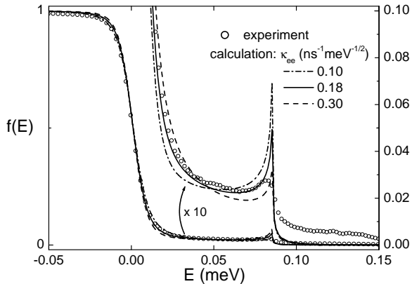
Fig. 9. Measured ( \circ ) distribution function f_{\frac{1}{4}}(E) in the new Relax experiment using sample AgXII40 depicted in FIG. 6, with the switch in position 2, and for U = -0.27 mV. The data are also shown magnified by a factor 10 (right scale). The solid line is a numerical solution to the Boltzmann equation with boundary condition given by EQ. (9), using as prefactor for the Coulomb interaction \kappa_{ee} = 0.18 \text{ ns}^{-1} \text{ meV}^{-1/2} . The two dot-dashed lines show that other values of \kappa_{ee} produce markedly worse fits to the data.
