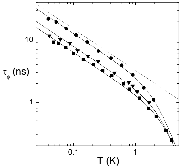
Fig. 2. Phase coherence time vs temperature in samples Ag(6N)a (■), Ag(6N)b (▼), and Ag(6N)c (●), all made of 6N sources. Continuous lines are fits of the data to EQ. (1). The quantitative prediction of EQ. (2) for electron-electron interactions in sample Ag(6N)c is shown as a dashed line.
