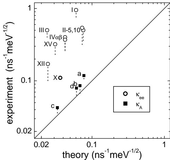
Fig. 4. Comparison of the experimental prefactor with the theoretical prediction EQS. (2),(4),(5), for weak localization experiments (■) and energy relaxation experiments (○). If we assume that a small amount of magnetic impurities is present in the WL samples, the fit values of \kappa_A can be reduced down to the bottom of the dashed lines below the squares. Similarly for the Relax experiments, if we assume that magnetic impurities are present, we obtain a range of values of \kappa_{ee} compatible with the data, represented as a dashed line below the \circ . The behavior of sample AgX20 was measured in a magnetic field, allowing us to place an upper bound on the concentration of magnetic impurities, and hence to rule out the possibility of reducing the value of \kappa_{ee} more than 15%. Thus, this data point is represented as a bold circle without any dashed line.
