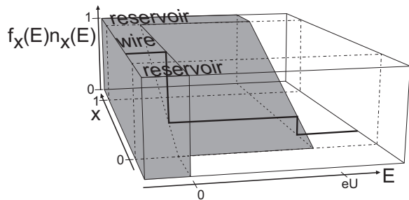
Fig. 1. Schematic diagram showing the spatial and energy dependence of the distribution function f_x(E) of QPs driven out-of-equilibrium by the voltage U using the geometry of FIG. 6 with the switch in position 1. The surrounding box shows the uniform density of states in the metal and the gray volume shows the occupied states whose normalized density is f_x(E)n_x(E) . The thick line shows a typical double step distribution function at x = 1/4 as in FIG. 7.
