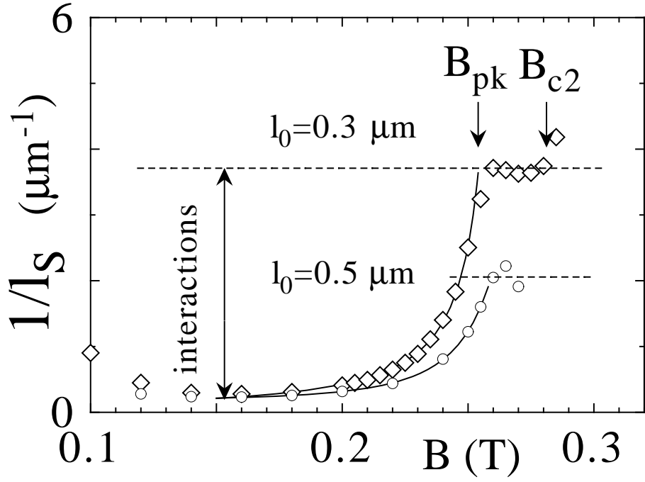
Figure 4: The slippage length l_S(B) for a vortex array at a rough surface. It is deduced from the L_S data according to l_S = L_S \mu_0 \epsilon / B in Eq.(1). The effect of vortex interactions in the collective-pinning regime below B_{pk} is visible as a suppression of 1/l_S(B) . Solid lines are power-law fits.
