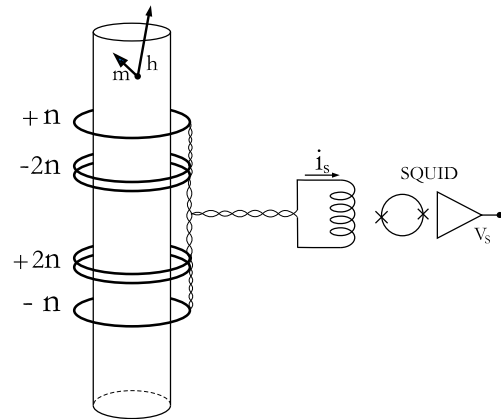
FIG. 1: Schematic of the basic circuit for noise measurement. In order to maximize the coupling factor between the sample and the Pick Up coil, a long cylinder (4 cm long, 4 mm wide) is used. The third order gradiometer being 2.2 cm long 5.5 mm wide, this size insures almost the best possible coupling factor, as any contact between the PU-coil and the sample must be avoid to allow the temperature regulation.
