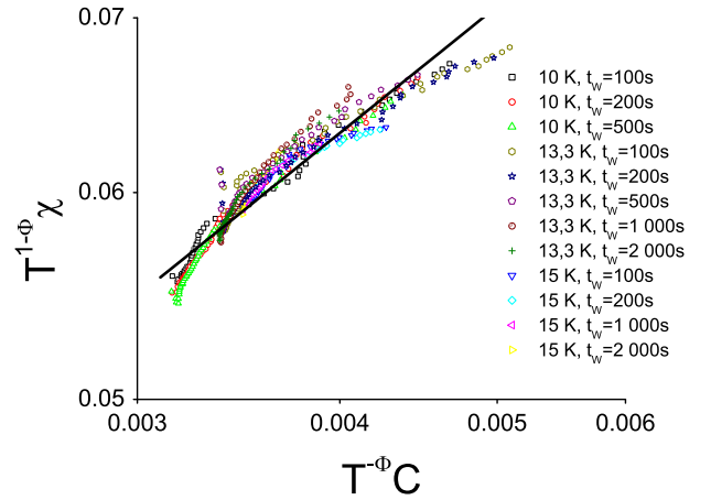
FIG. 7: Scaling of the aging parts of the FDT-diagram following equation 27. The straight line shows the result predicted by this equation.
