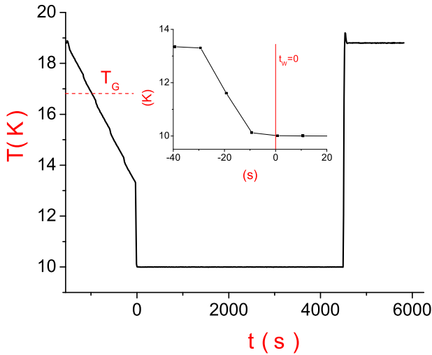
FIG. 4: A typical thermal history of the sample for a 4,500 record at 10 K. In inset, detail on the crucial part, the last 3 K's cooling.
