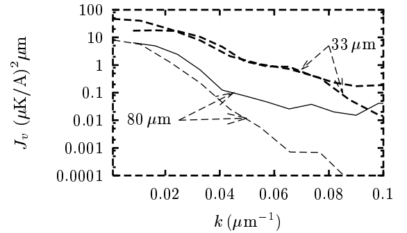
FIG. 3: Potential spectral density J_v = 1/(2\pi I^2) \int_{-\infty}^{\infty} (V_z(z)V_z(z+u))e^{iku} du at 33 \mu\text{m} from the wire (fat lines) and at 80 \mu\text{m} from the wire (thin lines). Solid lines : potential measured using cold atomic clouds. Dashed lines : potentials calculated from the measured geometric fluctuations of the edges of the wire. These estimations of the spectral density are made with the Welch algorithm [14] using windows half the size of the total explored region ( 1.6 \text{ mm} ).
