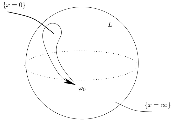
FIGURE 5. Holonomy compatibility
