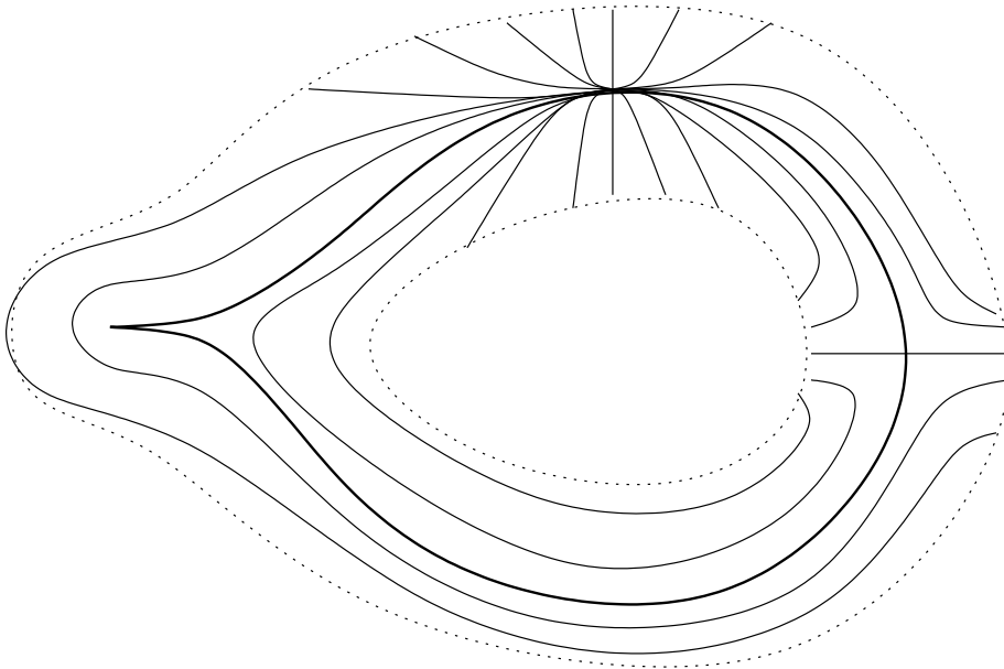
FIGURE 1. The geometry of normal forms from [14]
