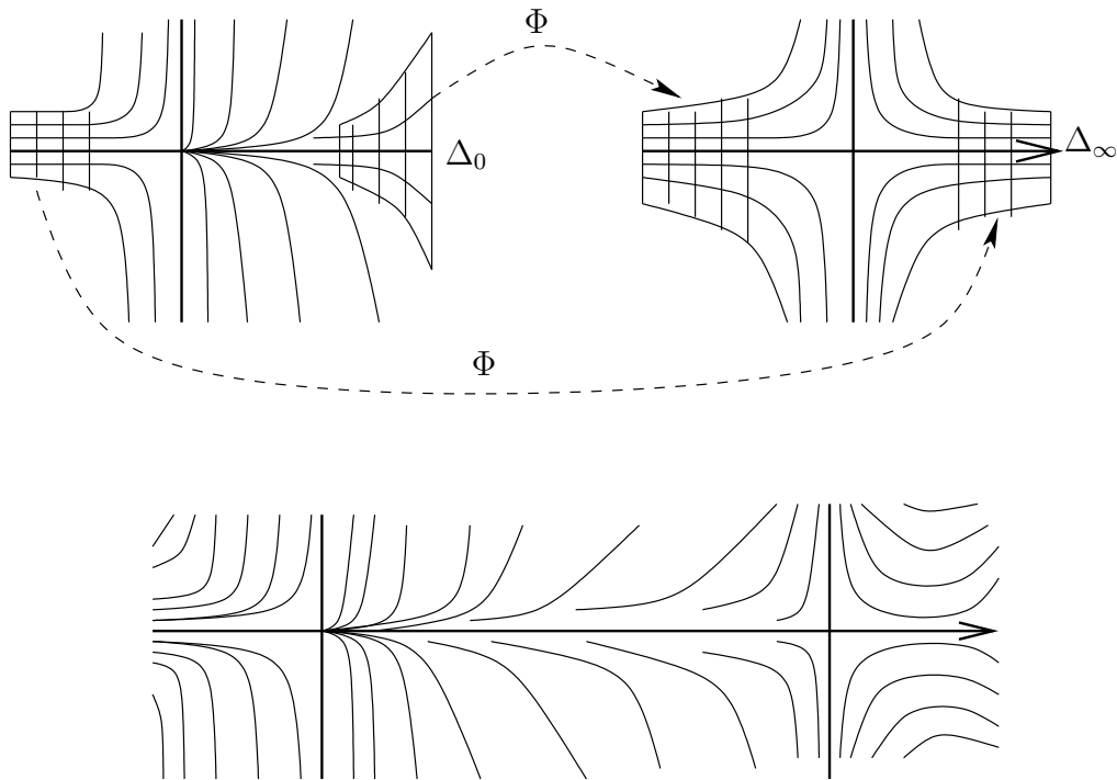
FIGURE 6. Gluing picture
