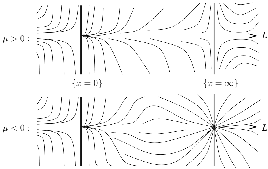
FIGURE 4. Geometry of the second normal form
