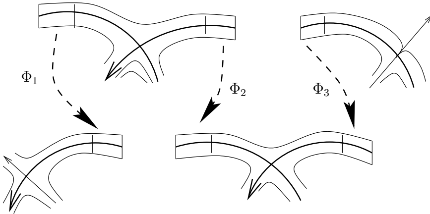
FIGURE 9. Gluing foliations along an exceptional divisor
