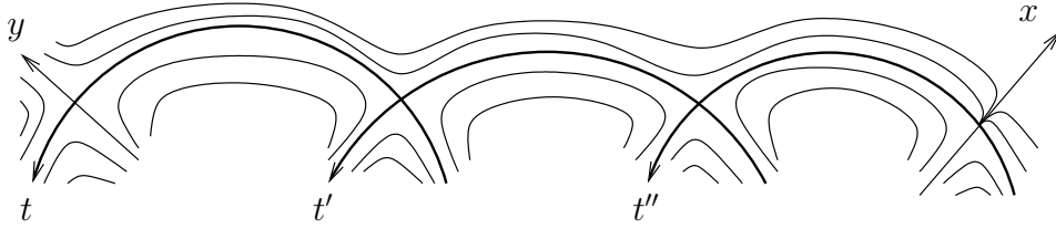
FIGURE 8. After 3 blowing-up
