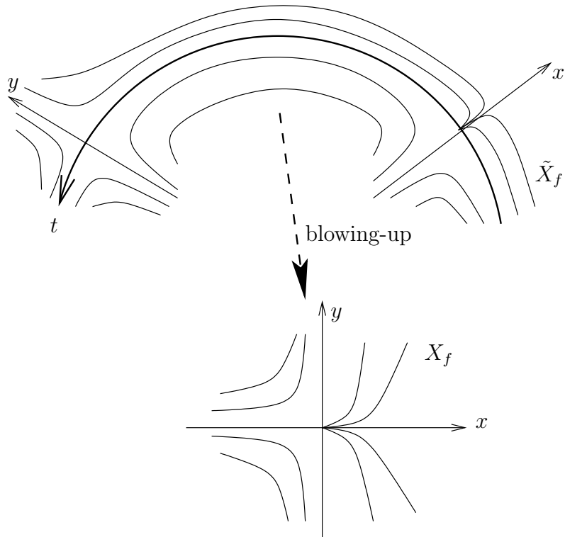
FIGURE 7. Blowing-up a saddle-node
