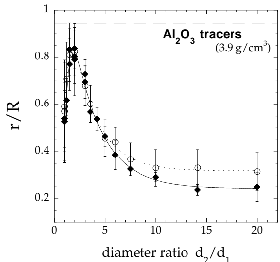
FIG. 11: Mean locations of 3-mm \text{Al}_2\text{O}_3 beads in a bed of small Glass beads: ( \circ ) 50 beads (3%), ( \diamond ) 10 beads (0.6%). Standard deviations of the distributions of the locations are represented as errors bars. The use of a larger amount of tracers slightly shifts r/R to larger values, but only at large diameter ratios. It also increases the standard deviations. The curve for 0.6% is the fit used in fig. 18.
