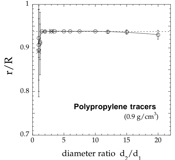
FIG. 4: Mean locations of 3-mm Polypropylene beads in a bed of small Glass beads: (O) 50 beads (corresponding to 3% volume fraction), ( \times ) 17 beads (1%). Standard deviations of the distributions of the locations are represented as errors bars. All beads touching the periphery corresponds to r/R=0.938 .
