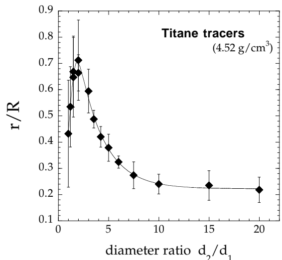
FIG. 12: Mean locations of 3-mm Titane beads in a bed of small Glass beads: ( \diamond ) 10 beads (0.6%). Standard deviations of the distributions of the locations are represented as errors bars.
