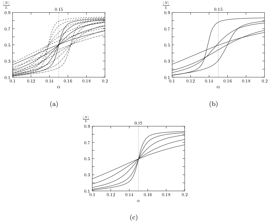
Figure 1: Mean density \langle N \rangle / L versus \alpha for a sample of size 11, 21, 41, 81 and 161. In figure 1(a), the system size is increased by adding new sites at the center (procedure C), and 3 samples are shown. In figure 1(b), the size is increased by adding new sites on the sides (procedure B) and a single sample is shown. In figure 1(c), the pure case (all the p_i = 1 ) is shown for comparison. The dotted line shows on the three figures the transition point of the pure TASEP.
