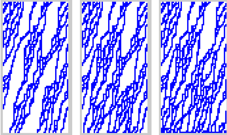
Figure 12. Evolution of ECA 46 for \alpha = 0.40 and d_{ini} = 0.30 (left) 0.50 (center) 0.80 (right)
