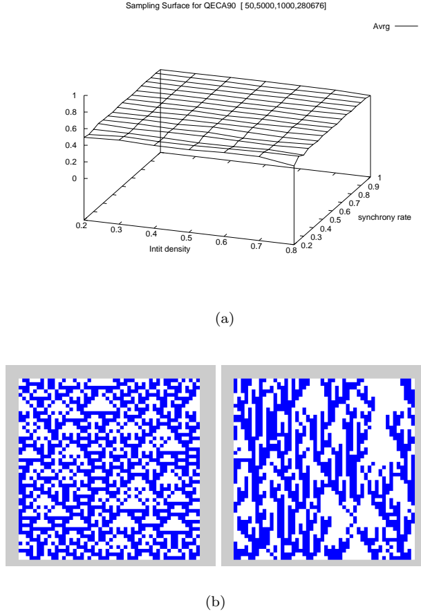
Figure 4. (a) An example of horizontal surface : ECA 90 (b) Evolution of ECA 90 : (left) \alpha = 1.0 (right) \alpha = 0.5 . In this space-time diagram and in the following the initial condition is obtained with a Bernoulli process with d_{ini} = 0.5 , the grid size is n = 50 , the time is from t = 0 to t = 49 .
