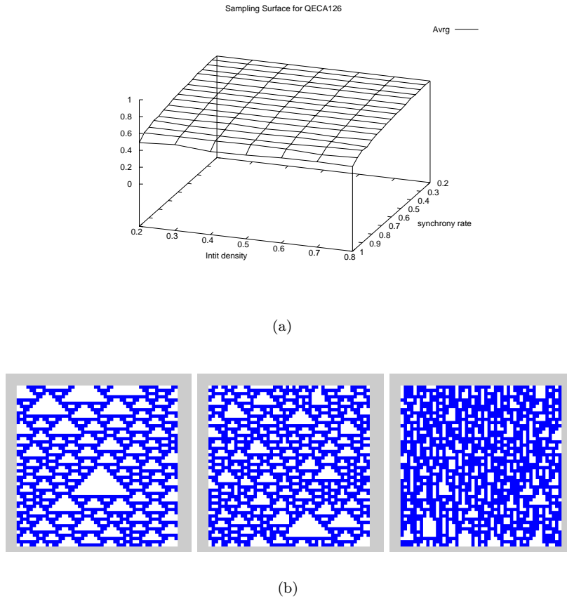
Figure 9. (a) An example of d_{ini} -invariant, \alpha -dependent sampling surface : ECA 126 ( \alpha -axis inverted). (b) Evolution of ECA 126 : (left) \alpha = 1.0 (center) \alpha = 0.9 (right) \alpha = 0.5 .
