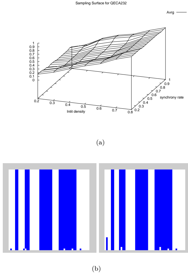
Figure 5. (a) An example of d_{ini} -dependent, \alpha -invariant sampling surface : ECA 232 . (b) Evolution of ECA 232 : (left) \alpha = 1.0 (right) \alpha = 0.5 . A tight examination of the configuration shows that the width of the second white band is larger in the left diagram.
