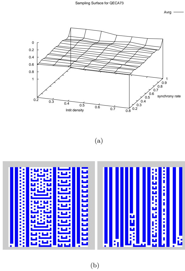
Figure 7. (a) An example of surface with a discontinuity at \alpha = 1.0 and noise for \alpha < 1.0 : ECA 73 (z-axis inverted for allowing the display of discontinuity at \alpha = 1 ). (b) Evolution of ECA 73 : (left) \alpha = 1.0 (right) \alpha = 0.8 .
