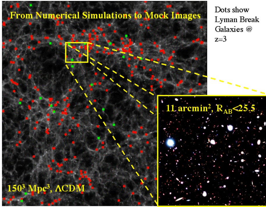
Figure 2: simulation from GALICS 11 of the cosmic web at z=3 . Red and green points shows that LGBs are correlated with the filaments. Small fields of view would lead to strong cosmic variance when studying physical properties of distant galaxies.
