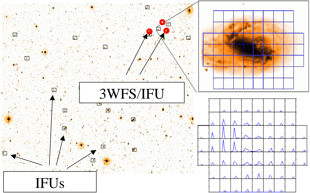
Figure 3: a schematic view of the FALCON concept with several IFU in a wide field ( \Phi=25 \text{ arcmin} ). Each IFU integrates an AO button for correction and is coupled with 3 WFS buttons which provide a WF reference at 3 nearby R<16 stars. Each individual IFU provides 62 spectra per galaxy at a spatial resolution of \sim 0.25 \text{ arcsec} (sampling \sim 0.1 \text{ arcsec} ).
