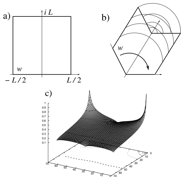
Fig. 1: a) Conformal mapping of the infinite complex plane inside a square w . b) Sketch which shows how the boundary conditions (BC) follow from the folding (“pillow” geometry). c) Example of the profile of the correlation function between the upper right corner and other points in the square with these particular BC.
