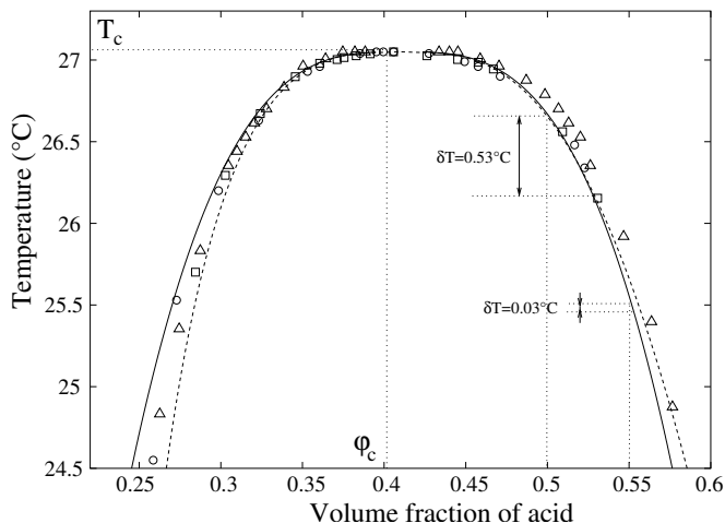
FIG. 1: Phase diagram ( \phi_{acid}, T ) of the isobutyric acid-water mixture from Woermann et al. [13] ( \circ ), Chu et al. [14] ( \square ), Zhuang et al. [15] ( \triangle ), Krall et al. [16] (dashed line) and Andrew et al. [17] (solid line). The critical temperatures have been matched to ours : T_c=27.05^\circ\text{C} . Our shallowest and deepest quenches are also represented.
