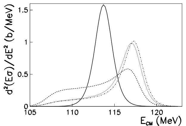
FIG. 3. Barrier distribution for the reaction ^{24}\text{Mg}+^{208}\text{Pb} i) assuming spherical nuclei (solid line); ii) considering a prolate deformed ^{24}\text{Mg} ( \beta_2 = 0.4 ) and the a.o.f. (dashed line); iii) and including reorientation with (dotted-dashed line) and without the rotational energy (dotted line).
