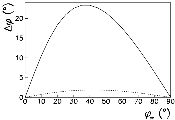
FIG. 1. Classical calculations (started at D_\infty = 241 fm) of the reorientation \Delta\varphi of the projectile as function of its initial orientation \varphi_\infty for the reactions ^{24}\text{Mg}+^{208}\text{Pb} (solid line) and ^{154}\text{Sm}+^{16}\text{O} (dashed line) at the barrier.
