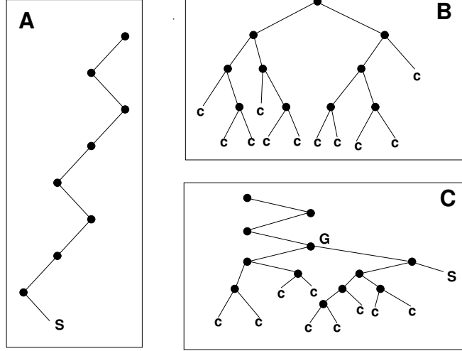
Fig. 2. Types of search trees generated by the DPLL solving procedure on random 3-SAT. A. simple branch : the algorithm finds easily a solution without ever backtracking. B. dense tree : in the absence of solution, DPLL builds a tree, including many branches ending with contradictory leaves, before stopping. C. mixed case, branch + tree : if many contradictions arise before reaching a solution, the resulting search tree can be decomposed into a single branch followed by a dense tree. G is the highest node in the tree reached by DPLL through backtracking.
